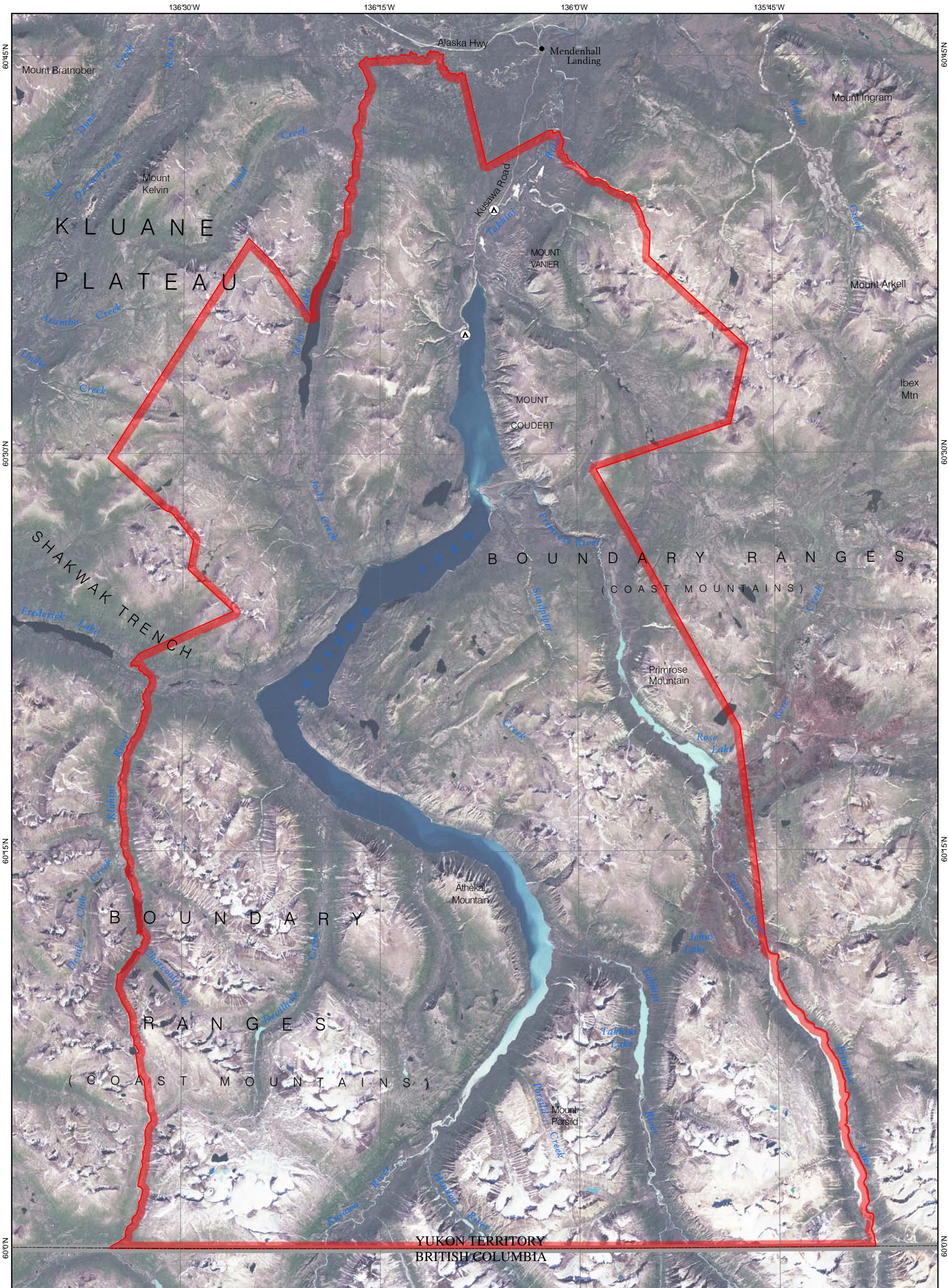
Map 2 Kusawa Territorial Park Landsat 7 Imagery Bands 1, 2, 3
